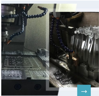
Ground Box Mould
